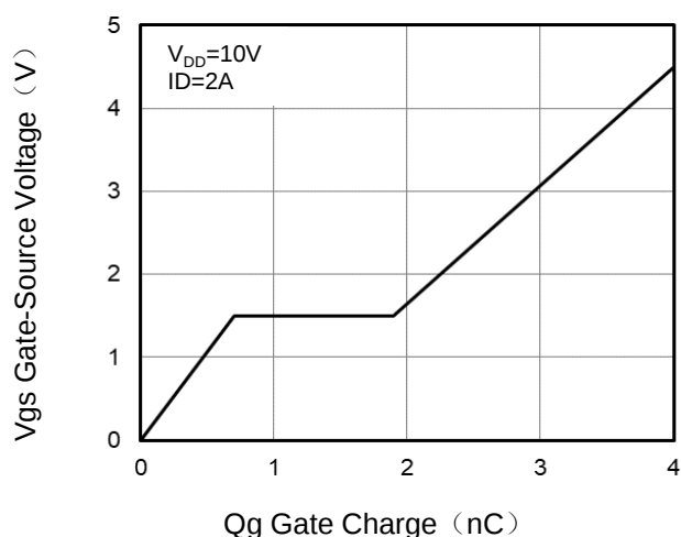
Figure 3. Gate Charge
