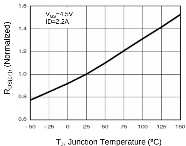
Figure 7. Drain-Source On-Resistance
